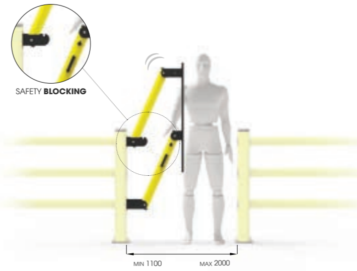
LIFT GATE 150
